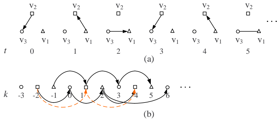
Fig. 1. Interaction topologies of an asynchronous system and its associated iteration graph. Nodes -3, -2, -1 denote initial conditions of agents v_3, v_2, v_1 , respectively.
